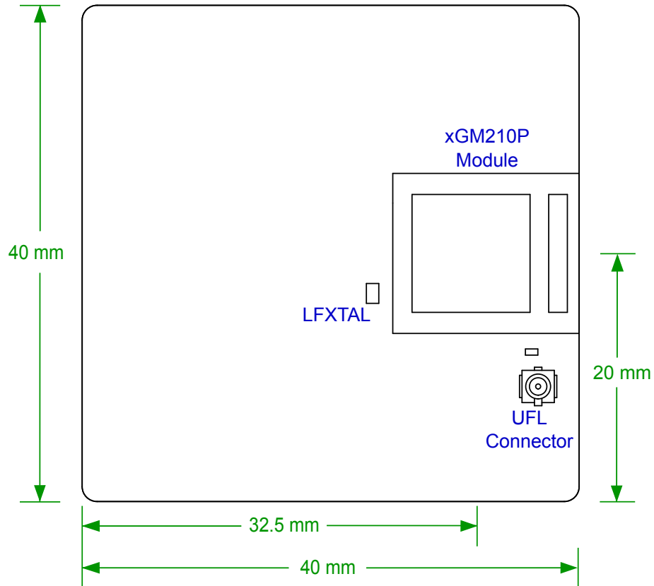
Figure 4.1. BRD4308D Top View
