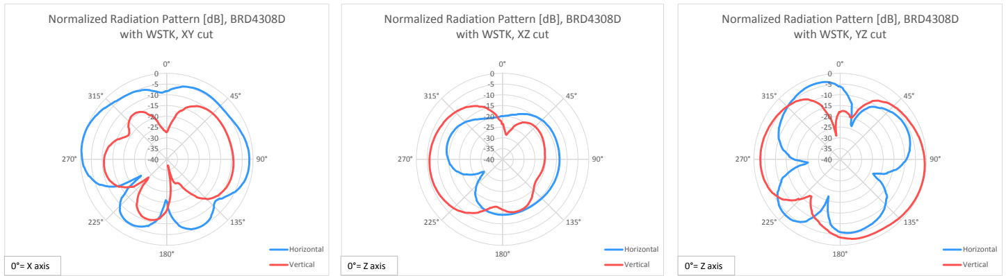
Figure 6.3. Normalized Antenna Pattern of the BRD4308D with the Wireless Starter Kit Mainboard
