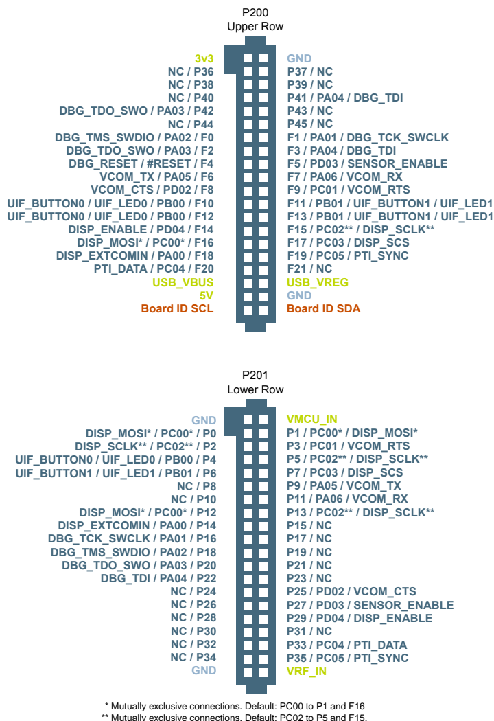
Figure 2.1. BRD4308D Radio Board Connector Pin Mapping
