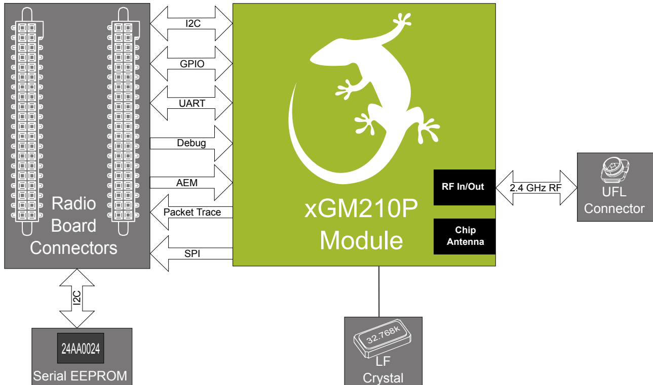
Figure 3.1. BRD4308D Block Diagram
