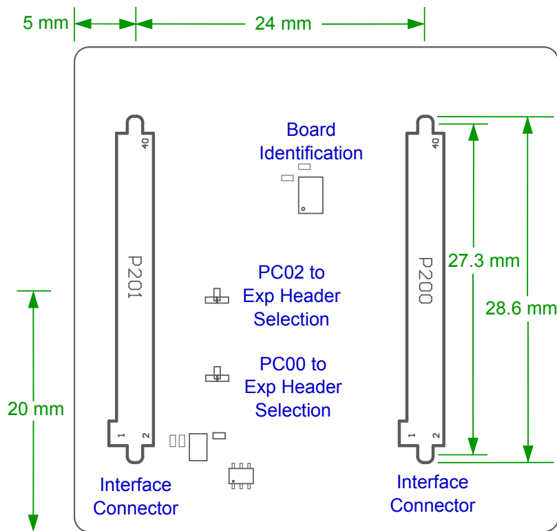
Figure 4.2. BRD4308D Bottom View
