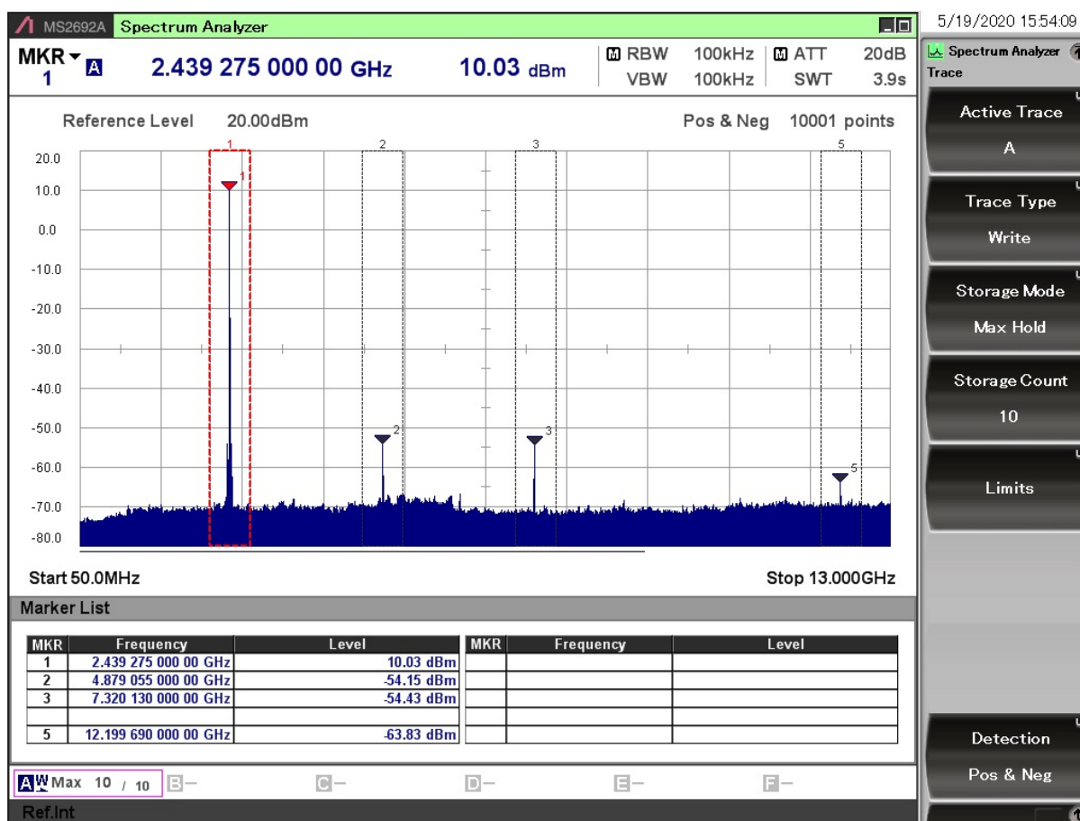
Figure 6.1. Typical Output Spectrum of the BRD4308D
