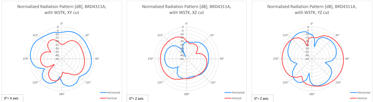
Figure 6.2. Normalized Antenna Pattern of the BRD4311A with the Wireless Starter Kit Mainboard
