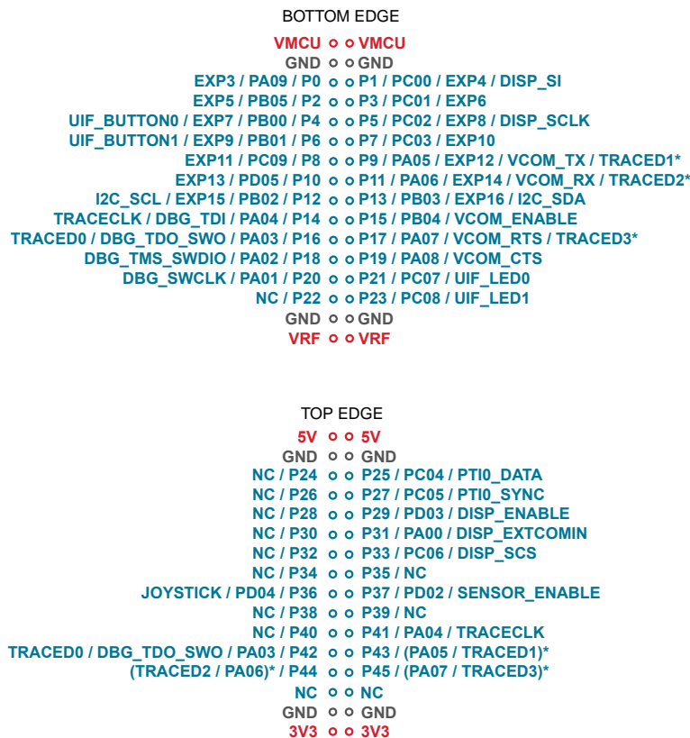
Figure 3.4. Wireless STK Mainboard (BRD4001A) Breakout Pad Pin Mapping
